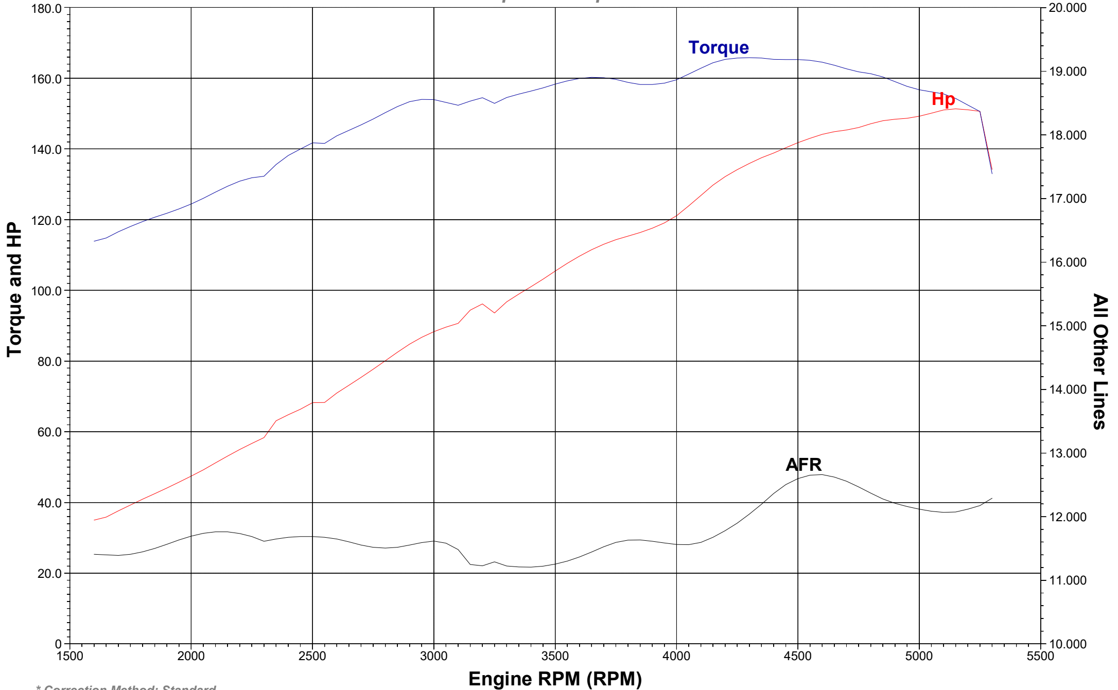
Peak Torque* and Hp* vs. RPM
